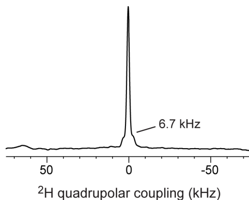
Figure S1. Static ^2\text{H} spectrum of \text{d}_{15} -Amt bound to M2(21-61) in the VM membrane at a P/L mole ratio of 1:30. The spectrum is still dominated by an isotropic peak, similar to the spectrum of the 1:15 sample shown in Fig. 4c , indicating that drug exclusion from the membrane is due to the high viscosity of the VM membrane rather than the high protein concentration.
