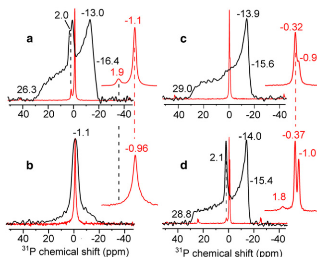
FIGURE 2 Static (black) and MAS (red) ^{31}\text{P} spectra of lipid membranes without and with M2. Inset expands the MAS spectra. (a) M2(21–61)-DMPC membranes at 303 K. (b) DMPC isotropic vesicles at 298 K. (c) M2TM-VM membranes at 303 K. (d) M2(21–61)-VM membrane at 303 K. An isotropic peak at about +2 ppm is observed in a and d .
