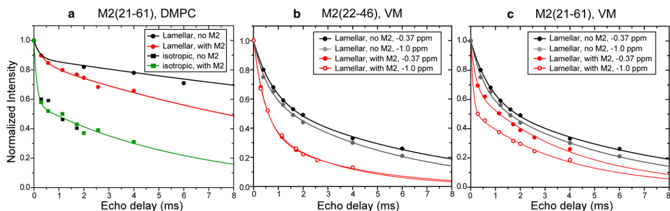
FIGURE 4 ^{31}\text{P} -detected ^1\text{H} T_2 relaxation decays without (black) and with (red and green) M2 at 298 K. (a) DMPC bilayers with and without M2(21–61). (b) VM membranes with and without M2(22–46). (c) VM membranes with and without M2(21–61).
