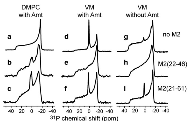
FIGURE 1 Static ^{31}\text{P} spectra of DMPC (a–c) and VM (d–i) membranes in the absence and presence of M2 at 303 K. (a, d, and g) Protein-free lipid bilayers. (b, e, and h) M2TM-containing membranes. (c, f, and i) M2(21–61)-containing membranes. The DMPC spectra (a–c) and the VM spectra (d–f) were measured on samples with Amt, whereas the VM spectra (g, h, and i) were measured on samples without Amt.
